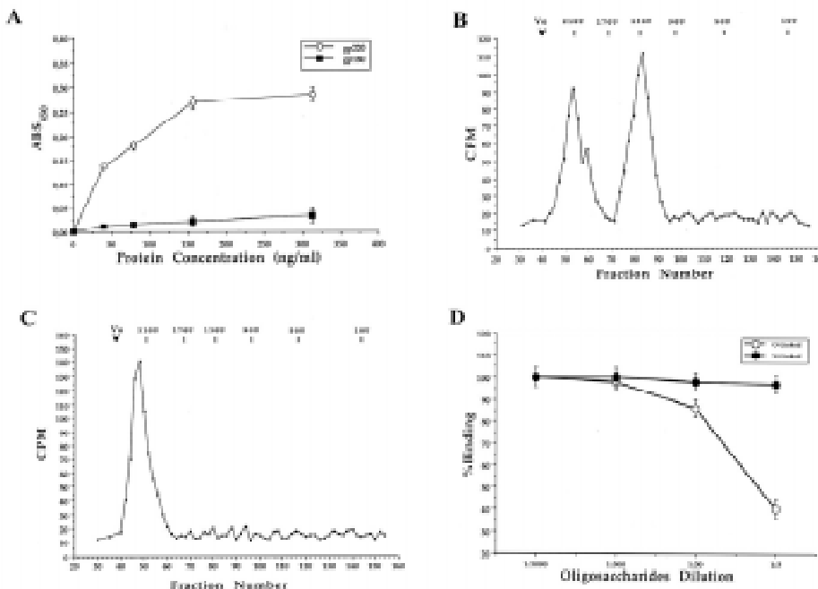
Fig. 6. The ligand molecule for sperm-egg interaction is gp273 and its O-linked chains play a key role in this interaction. (A) Binding of HRPO-conjugated coat glycoproteins to immobilized Unio sperm. (D) Differential effect of Biogel P4 purified gp273 N-linked (B) and O-linked (C) oligosaccharides on sperm binding to gp273.
