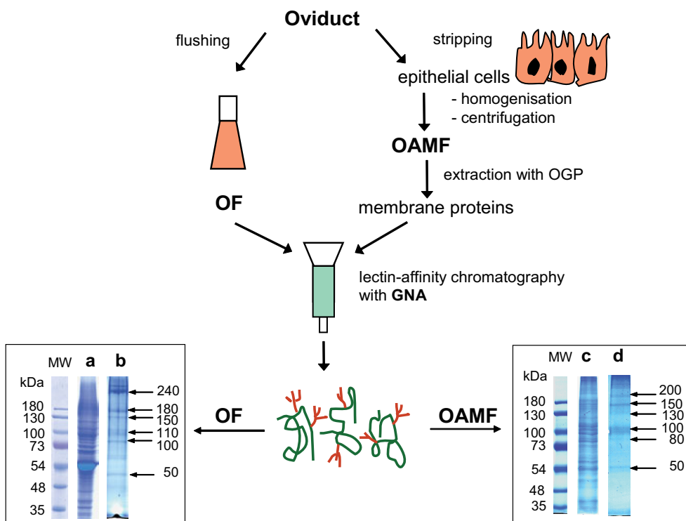
Fig. (3A). Strategy for isolation of the mannose-rich glycoproteins of the porcine oviduct. The oviductal fluid (OF) was isolated by flushing the oviducts with 0.15 M NaCl (Buhi et al., 1990), followed by centrifugation to separate cell debris and dialysis against water. The oviductal apical membrane fraction (OAMF) was isolated according to the method of Fazeli et al., 2003. Transmission electron microscopical examination verified the preferential occurrence of plasma membrane vesicles. The OAMF was solubilized in 1% OGP (octyl glucopyranoside) in phosphate-buffered saline pH 7.4 containing protease inhibitors. Affinity chromatography was performed on AffiSep-GNA-columns (0.75ml, Galab Technologies, Germany), which were run in PBS. GNA-binding proteins were released with 200mM \alpha -methyl-mannopyranoside in PBS. Insets: SDS-PAGE of OF and OAMF. Aliquots (5-20 \mu g) were subjected on 8% gels. Proteins were visualized with Coomassie-Brilliant Blue-staining.
