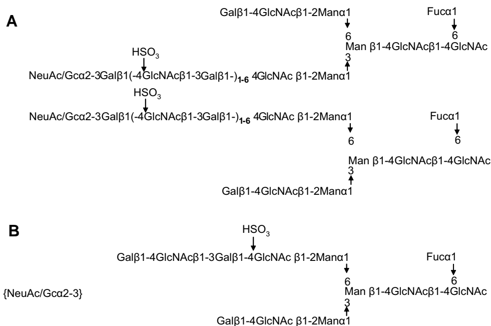
Fig. 7. Structures of the dominant sulfated N-glycans of the porcine zona pellucida. (A) The dominant bi-antennary acidic N-glycans of the isolated PZP3 family (ZPB/ZPC) according to Noguchi and Nakano (1992). (B) The major acidic N-glycan of the ZP glycoproteins of prepuberal pigs. To a minor extent this structure also exists in the sialylated form.
